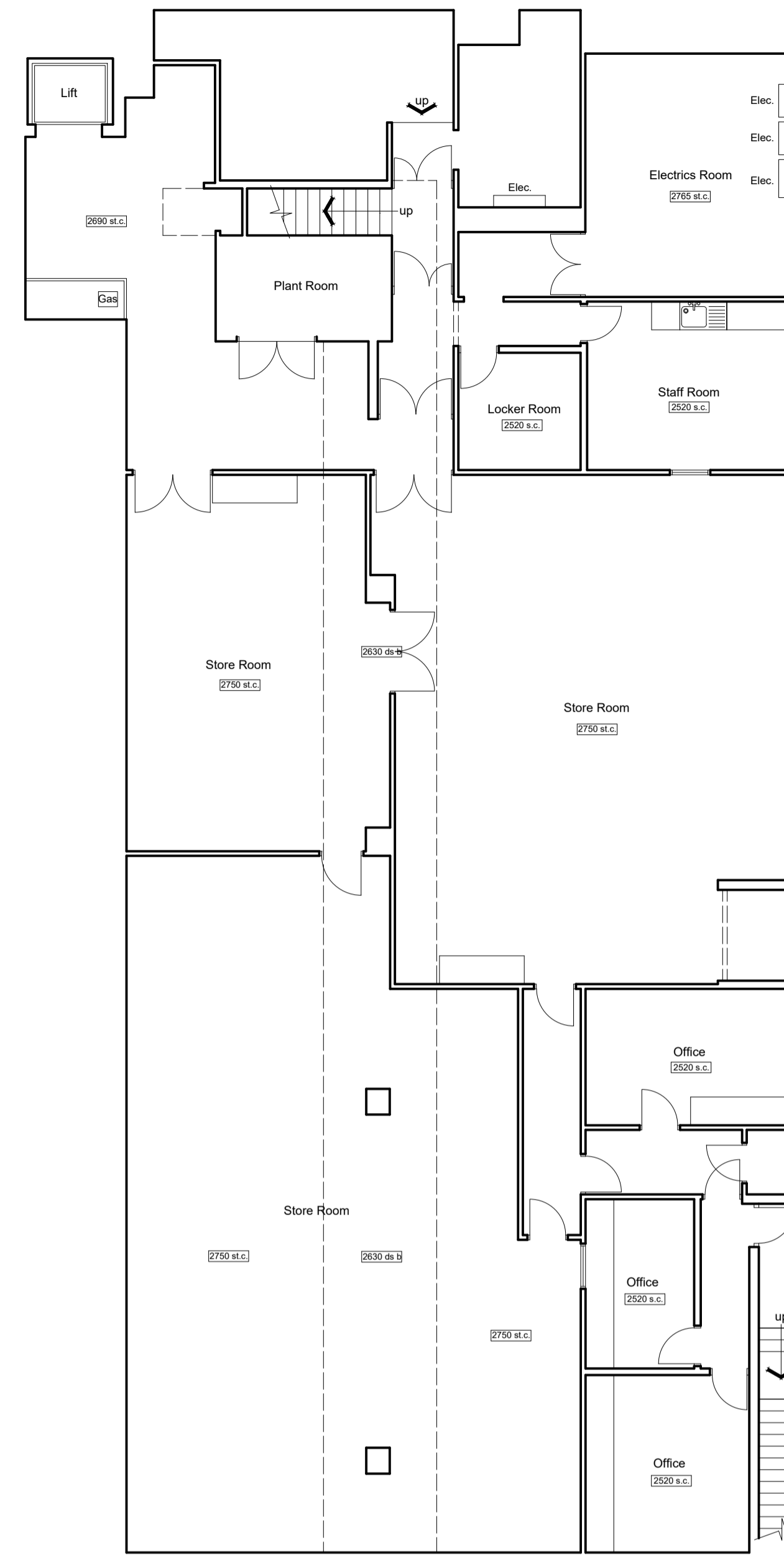
Basement Floor Plan
